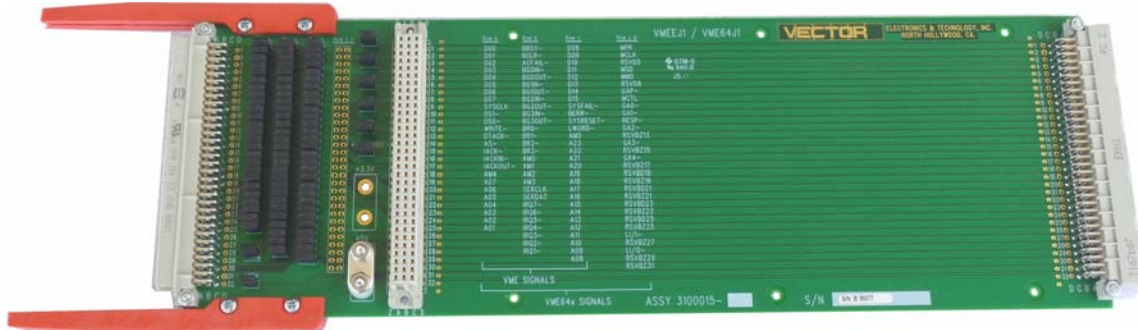
3U, VME J1 with 3-row, 96 positions DIN 41612 style connectors (click on image to enlarge)
